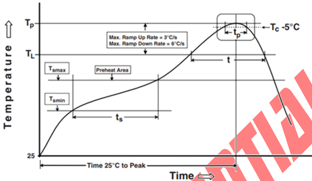
Figure 4 – Reflow
