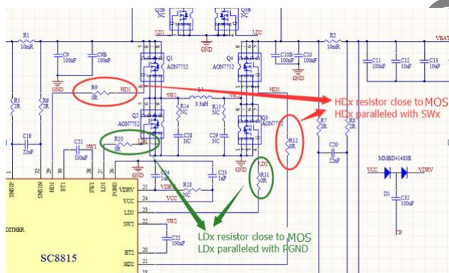
Figure 13 Schematic
